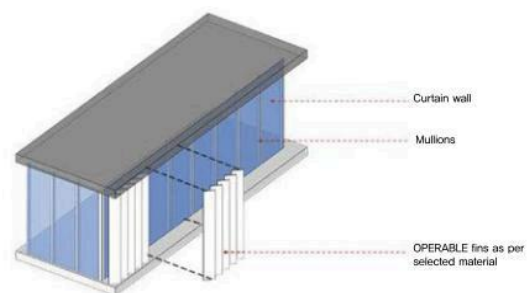
EAST WEST FACADE CURTAIN WALL WITH OPERABLE FINS
