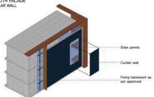
SOUTH FACADE SOLAR WALL
