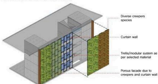
SOUTH FACADE CURTAIN WALL WITH PLANTER SCREENS
